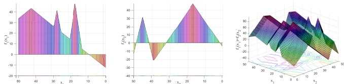
(a) 1-dimensional MPB with 3 peaks (b) 1-dimensional MPB with 2 peaks (c) 2D CMPB with 6 peaks by adding (a) and (b).
