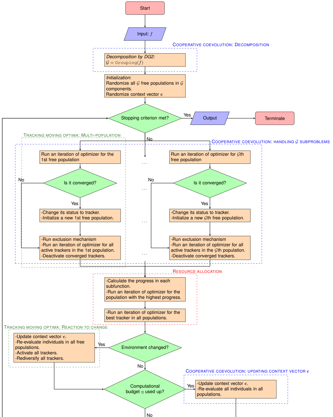
Fig. S-1. Flow chart of the proposed framework.
